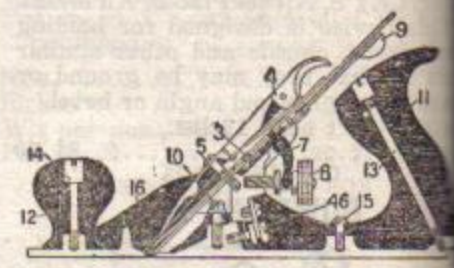
Sectional View of Bailey Iron Plane
