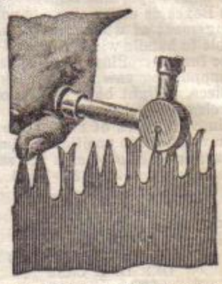
Set and swaging hammer.
