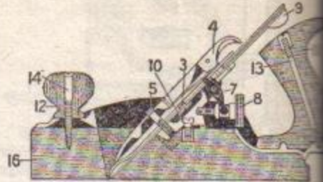
Sectional View of Bailey Wood Plane
