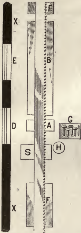
Fig. 1.—Showing proper position of table, etc., in front of windows E and D; XX being blank wall. A, anvil; B, leveling table; EF, continuation of bench; G, table holding hammers, etc.; H, position of operator at work; S, position of Roll Stretcher.
