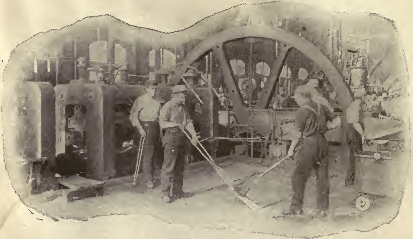
Ready for Rolling Long-Saw Plate.
