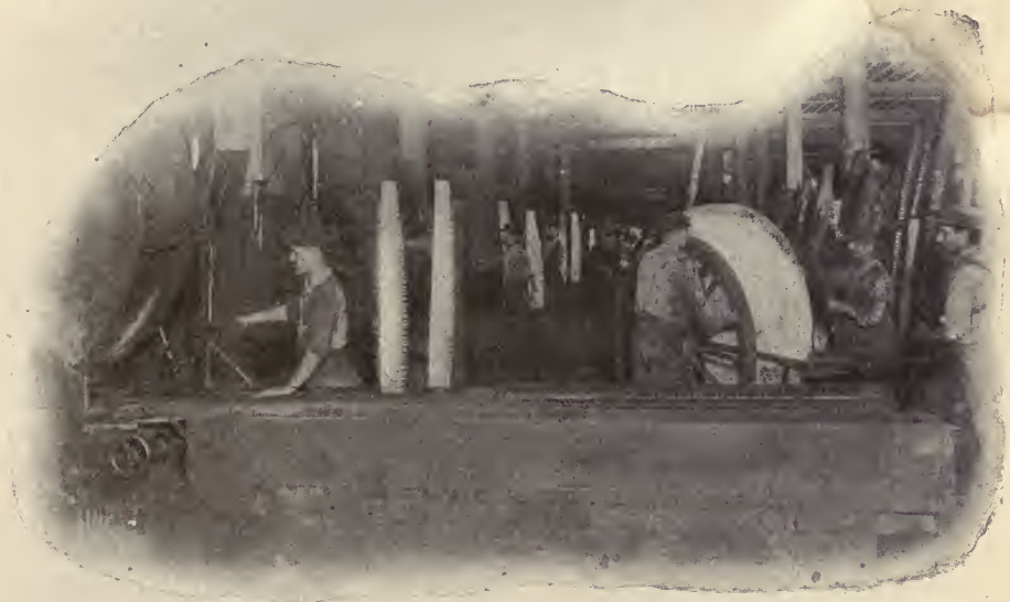
Grinding Long-Saws.
