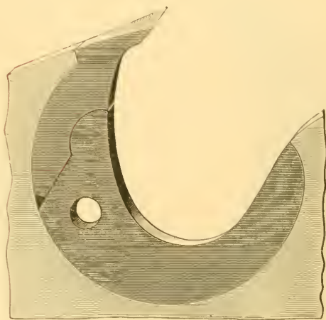
No. 4 CHISEL POINT. Full size of tooth.
