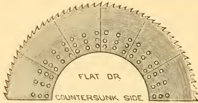
Left-Hand.
