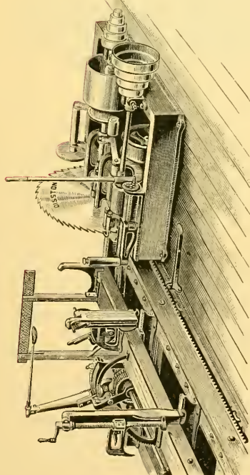
LEFT-HAND SAW.
