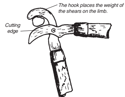
Lopping shears
