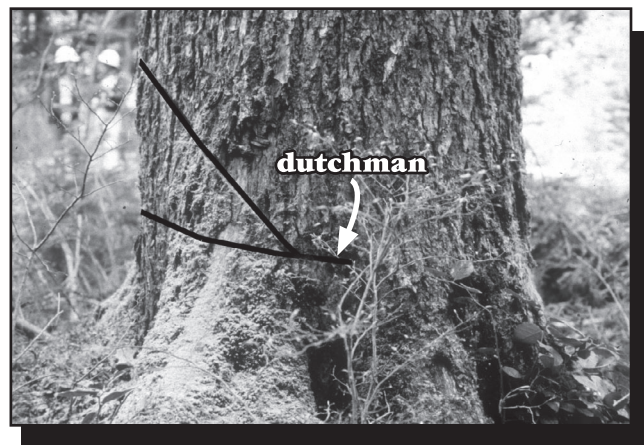
Figure 5-27—When the sloping cut and the horizontal cut do not meet exactly, a dutchman is formed. This kerf-wide cut makes the direction of the tree's fall harder to predict. It can also cause the tree to barber chair, lifting the log off the stump and placing the sawyers at great risk.
