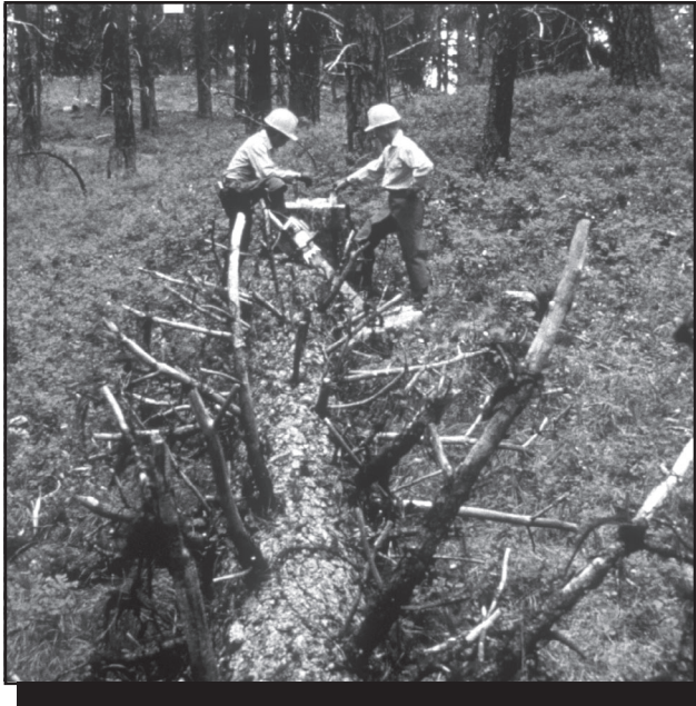
Figure 4-20—Look at the stump when critiquing a felling operation.
