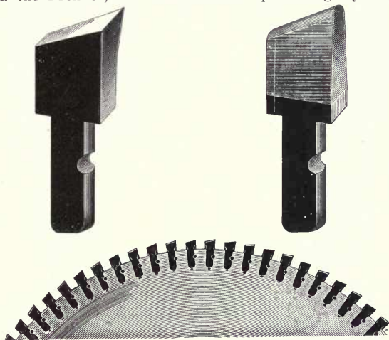
Regal Teeth, and Section of Saw
