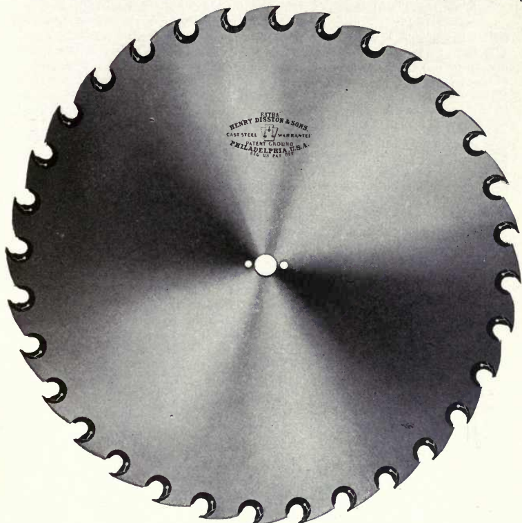
Inserted Tooth Circular Saw
