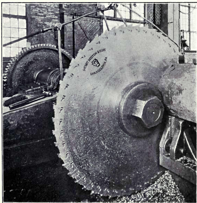
26-inch Blade, Bar Cold Saw Cutting Off Machine
