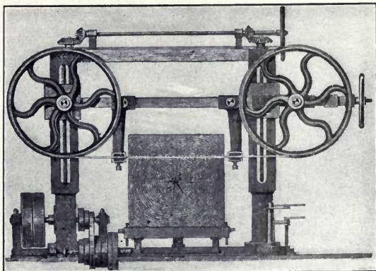
One of the first Horizontal Band-Saws
