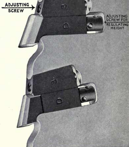
View of socket showing screw for regulating the height of tooth
