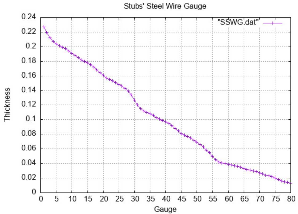
Figure 8: Stubs' Steel Wire Gauge Common Gauges.inc
