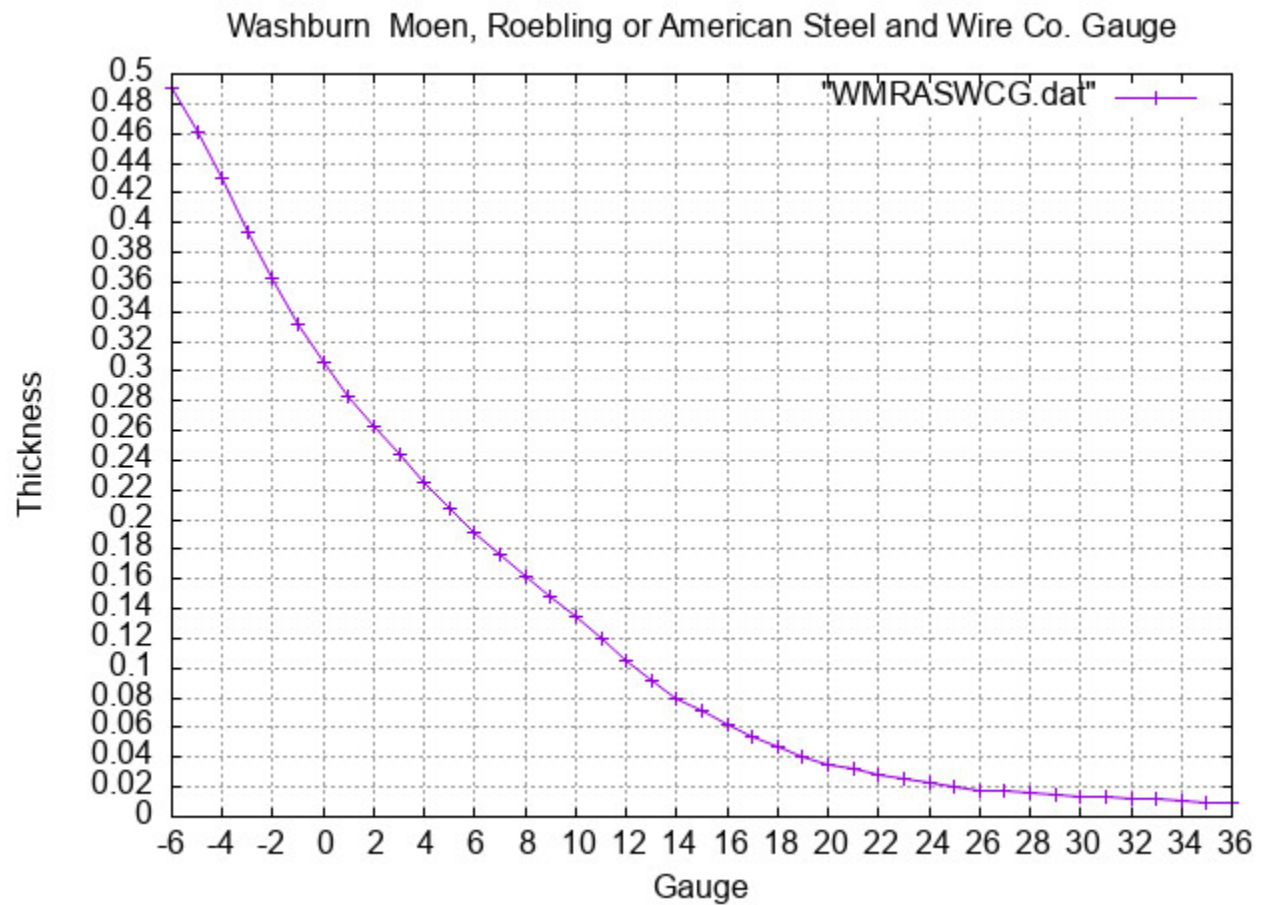
Figure 9: Washburn & Moen, Roebling or American Steel and Wire Co. Gauge Common Gauges.inc
