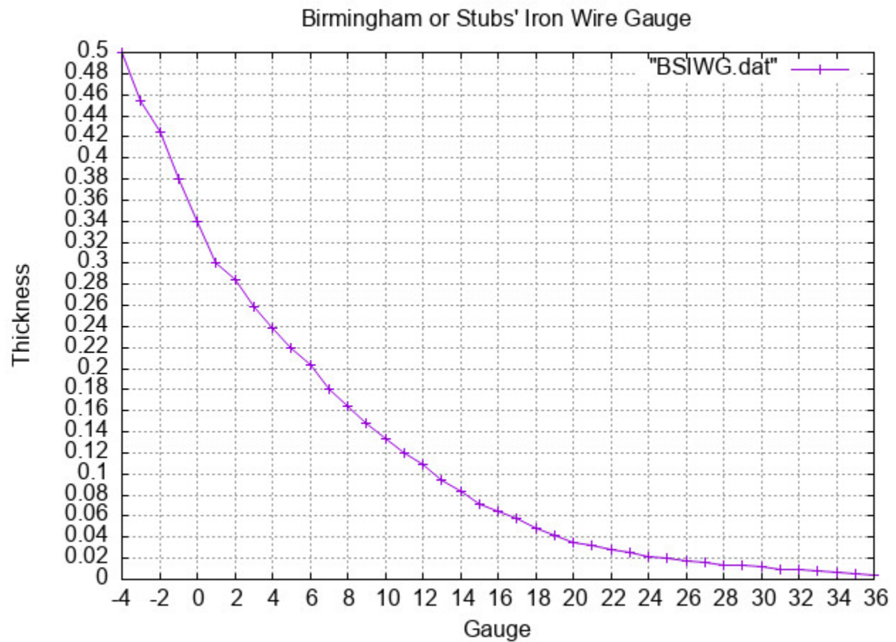
Figure 7: Birmingham or Stubs' Iron Wire Gauge Common Gauges.inc
