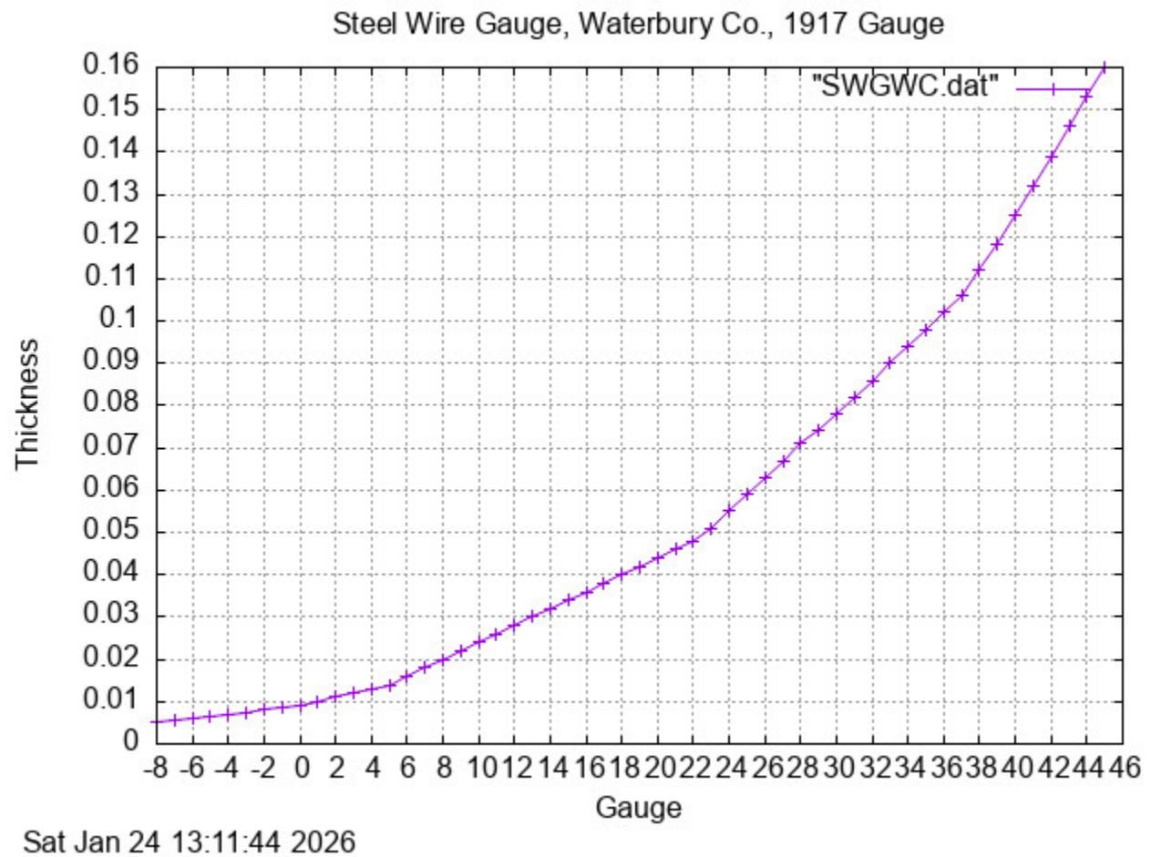
Figure 12: Steel Wire Gauge, Waterbury Co., 1917 Gauge Common Gauges.inc
