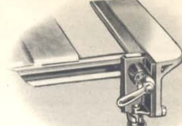
View of fence in rolled over position. This exclusive feature provides extra table space and allows you to get the fence out of the way for cross cutting without removing it from the machine.
