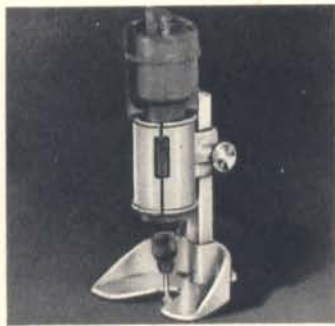
Router Stand
