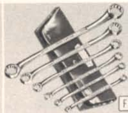
E F CRAFTSMAN 6-pc. Metric Wrench Sets. Forged; chrome plated. Plastic pouch. One each of sizes below. (E) 9 M 4450—Open end, 6-pc. Set, Shpg. wt. 1 lb. 11 oz. $5.79 (F) 9 M 4295—Box end, 6-pc. Set, Shpg. wt. 1 lb. 14 oz. $6.98
