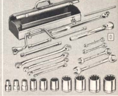
D CRAFTSMAN 25-piece Whitworth Wrench and Socket Set. \frac{1}{2} -inch square drive. Hot forged thin-wall sockets. Chrome plated. Set includes: ten 12-pt. sockets ( \frac{3}{16} , \frac{1}{4} , \frac{5}{16} , \frac{3}{8} , \frac{7}{16} , \frac{1}{2} , \frac{9}{16} , \frac{5}{8} , 1\frac{1}{16} , \frac{3}{4} W); two extension bars (6 and 10 in.); 18-in. speeder wrench; 15-in. flex handle; crossbar; 9\frac{3}{4} -in. reversible ratchet; four box-end and four open-end wrenches ( \frac{3}{4} x \frac{1}{2} , \frac{3}{4} x \frac{3}{16} , \frac{3}{8} x \frac{1}{16} , \frac{3}{8} x \frac{9}{16} W); tool box. 9 M 44096—Shpg. wt. 14 lbs. $32.95
