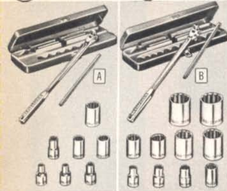
A CRAFTSMAN 10-piece Metric Socket Wrench Set. \frac{1}{2} -inch square drive. Hot forged thin-wall sockets get into tight places. Chrome plated. Set includes: seven 12-pt. sockets (9, 10, 12, 14, 17, 19, 22 mm.); 15-inch flex handle; crossbar; steel tool box. 9 M 43963—Wt. 4 lbs. 10 oz. $9.49
