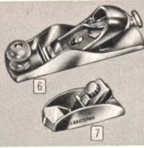
Block and Knuckle-joint Planes cut across grain
