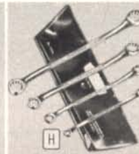
G H CRAFTSMAN 4-piece Whitworth Wrench Sets. Forged steel; chrome plated to resist rust. In handy plastic carrying pouch. The 4-piece sets include one each of the sizes listed in the table below. (G) 9 M 4368—Open end, 4-pc. set, Shpg. wt. 1 lb. 11 oz. $4.49 (H) 9 M 4296—Box end, 4-pc. set, Shpg. wt. 1 lb. 14 oz. $5.69
