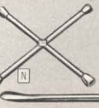
N CRAFTSMAN Cross-rim Wrench. Forged steel. For hex nuts. 16-inch arms. Has \frac{1}{8} , \frac{1}{4} and two \frac{3}{8} -in. openings. Chrome plated. 9 M 4472—Shpg. wt. 3 lbs. $1.98
