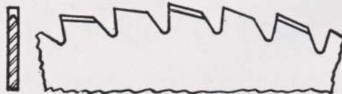
COPPER SLITTING TOOTH — each alternate tooth is "V" shape on top
