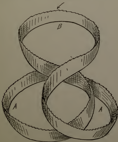
Fig. 105.—Coiling Band-Saw.
